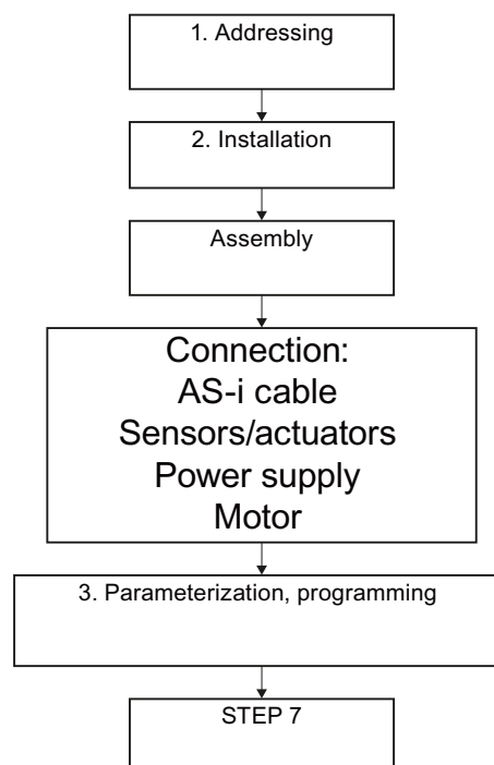
Figure 7-2 Commissioning procedure
