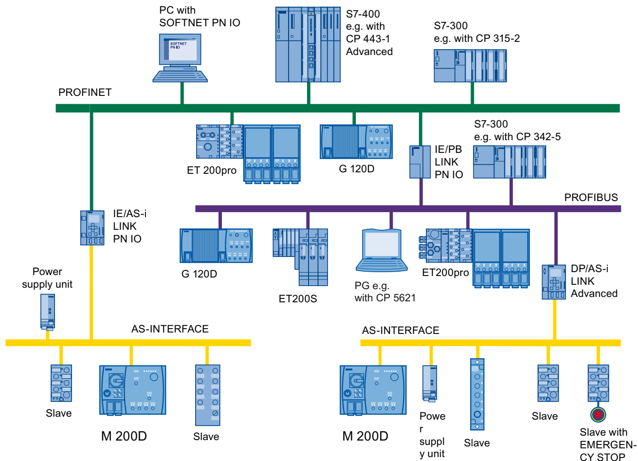
Figure 1-1 M200D: overview
