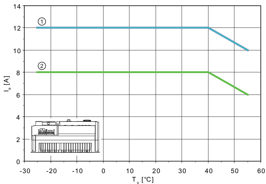
Figure 5-4 Derating for flat mounting
