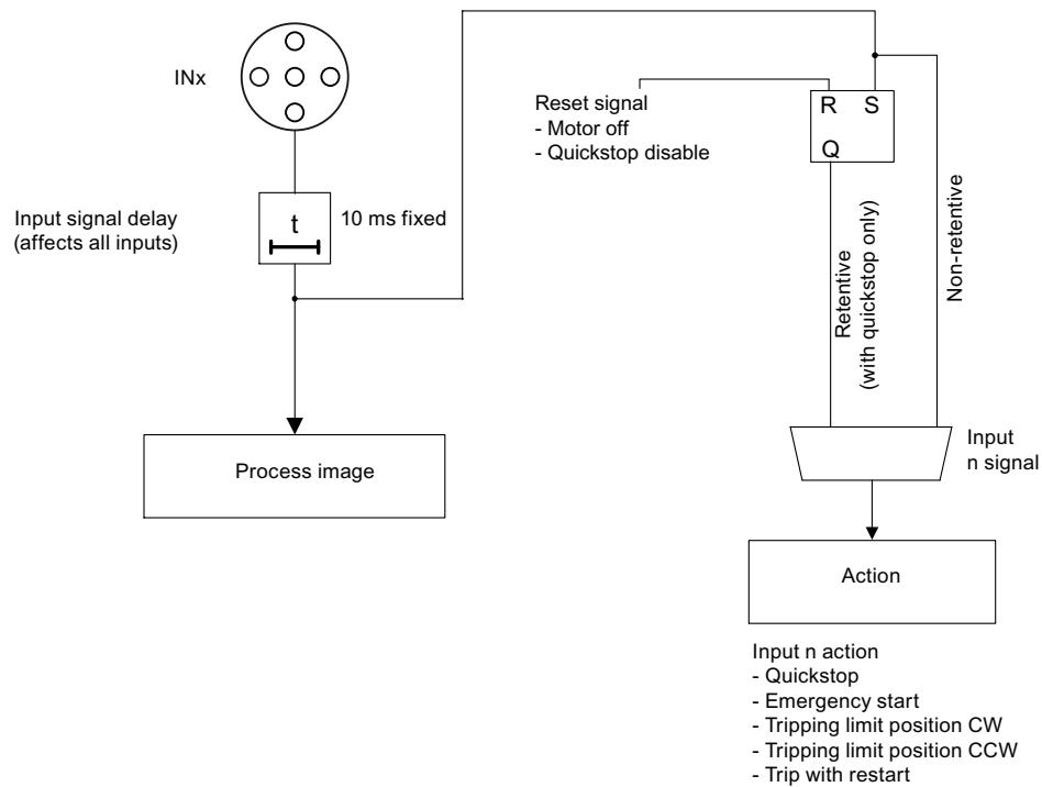
Figure 4-3 Overview of input parameters
