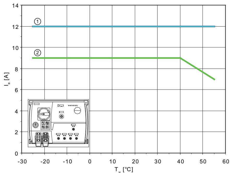
Figure 5-2 Derating for horizontal mounting
