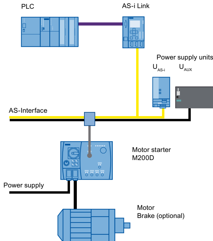
Figure 7-1 Minimum configuration of a motor controller
