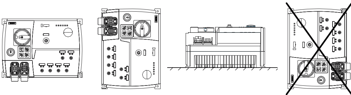
Figure 5-1 Installation positions: horizontal, vertical, flat; must not be positioned as shown on the right
