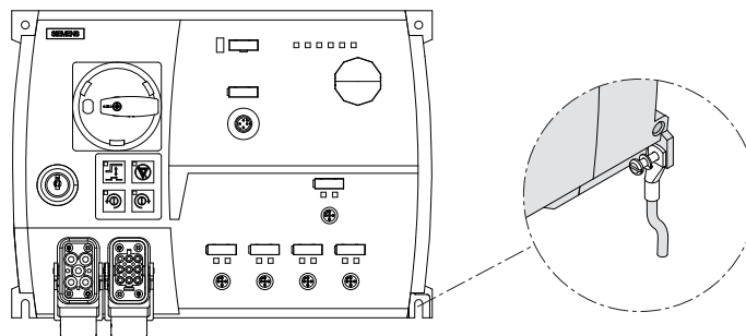
Figure 5-5 Connection for functional ground
