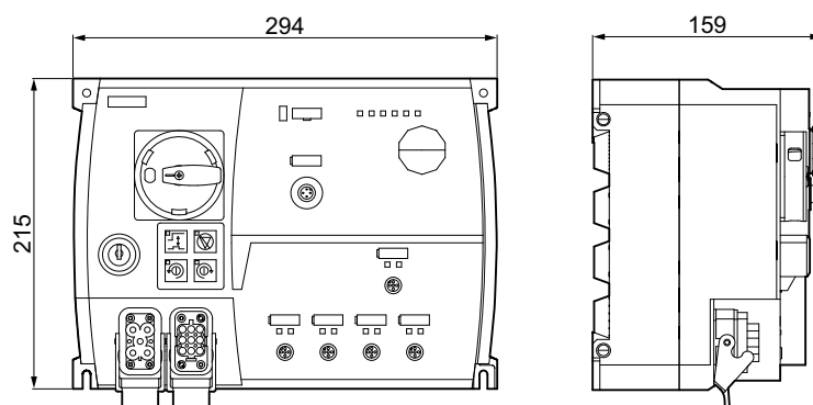
Figure 9-2 M200D AS-i motor starter without protection guard
