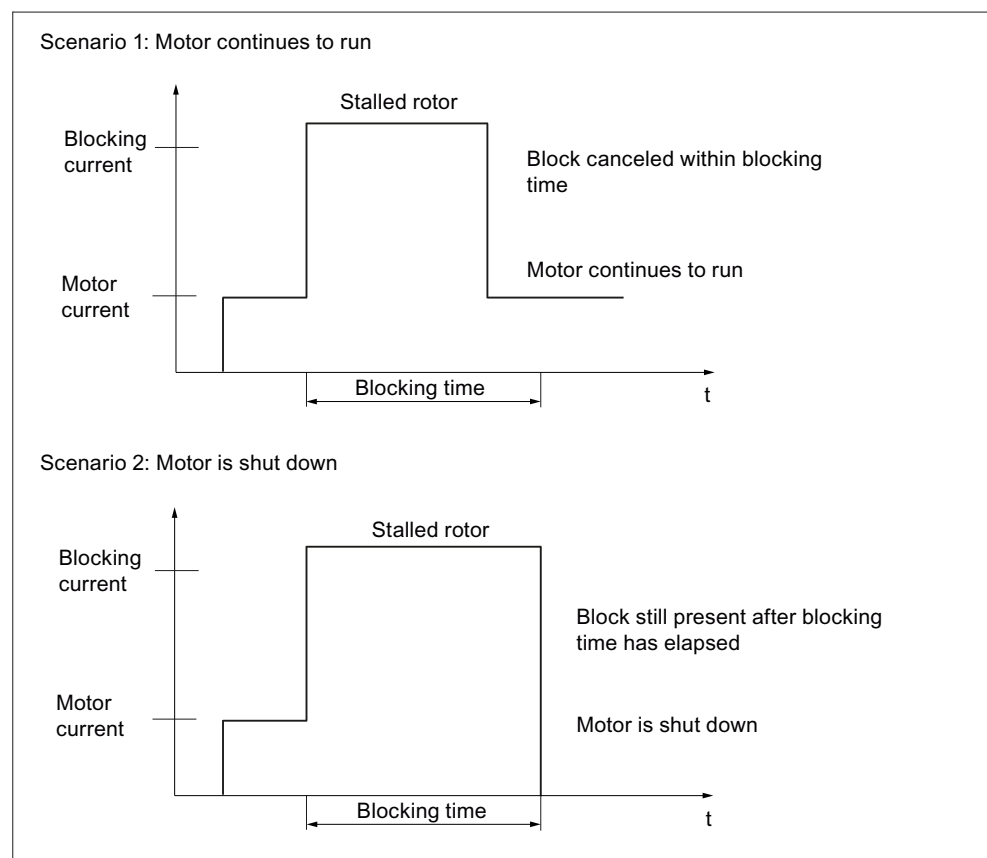
Figure 4-2 Blocking protection principle
