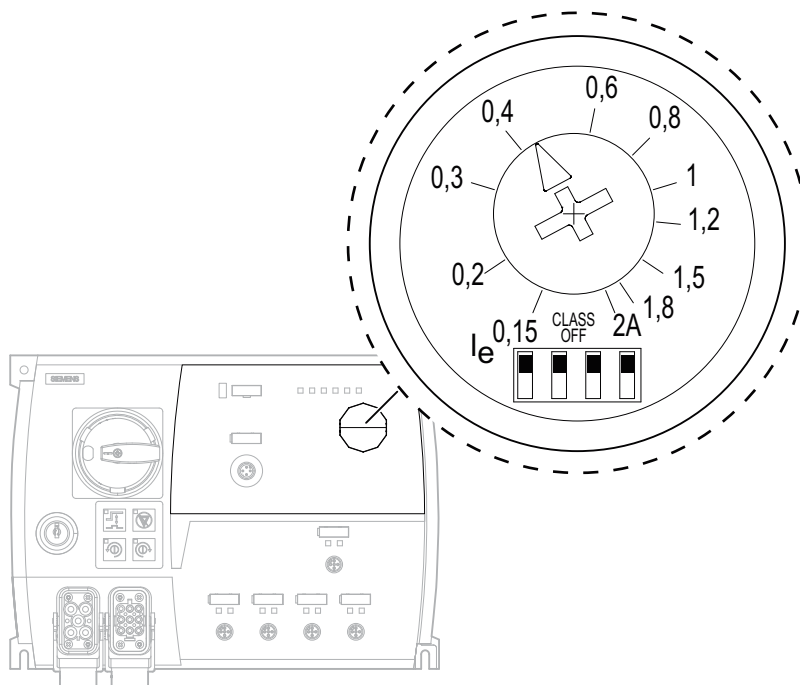
Figure 6-1 Rotary coding switch with 2 A scale
