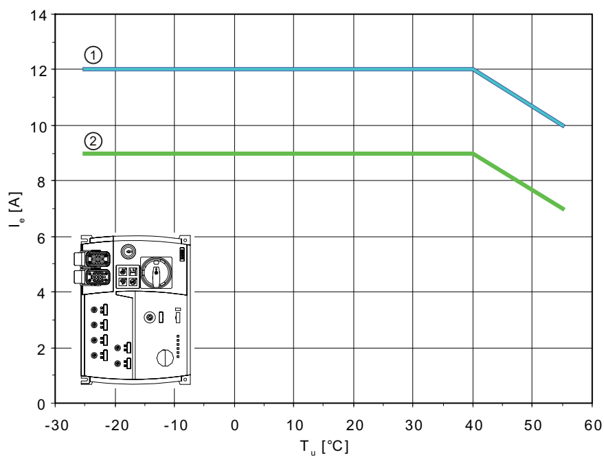
Figure 5-3 Derating for vertical mounting
