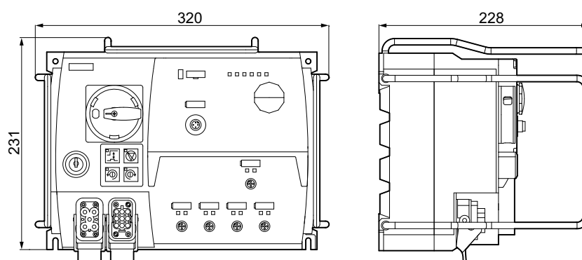
Figure 9-3 M200D AS-i motor starter with protection guard
