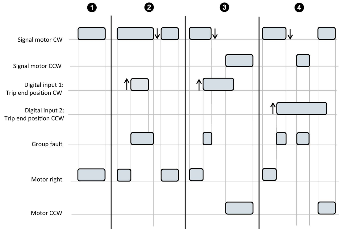
Figure 3-18 Example of trip end position CW
