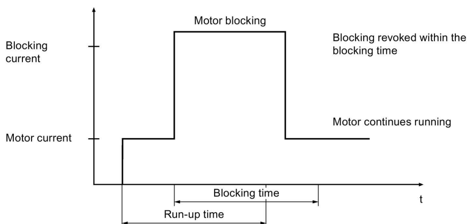
Case 1: Motor continues running
