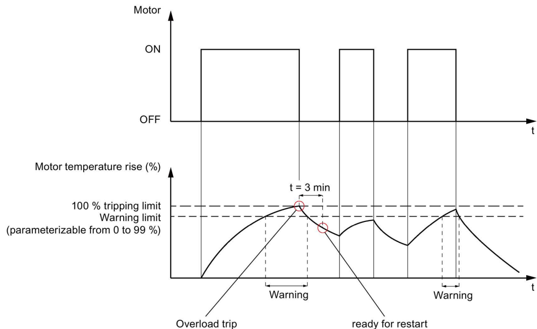
Figure 3-5 Principle of operation
