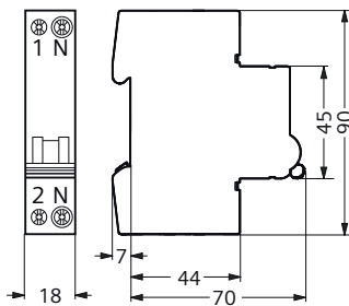
1P+N (N pole, right)
