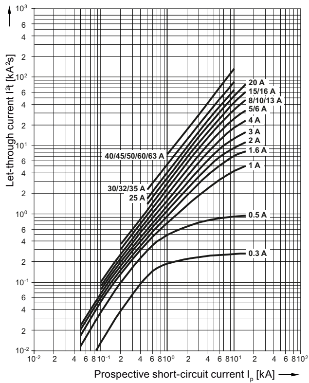
Characteristic D
