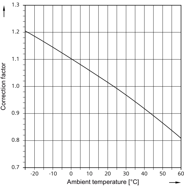
Correction factors regarding delayed tripping current at different ambient temperatures for 5SY1
