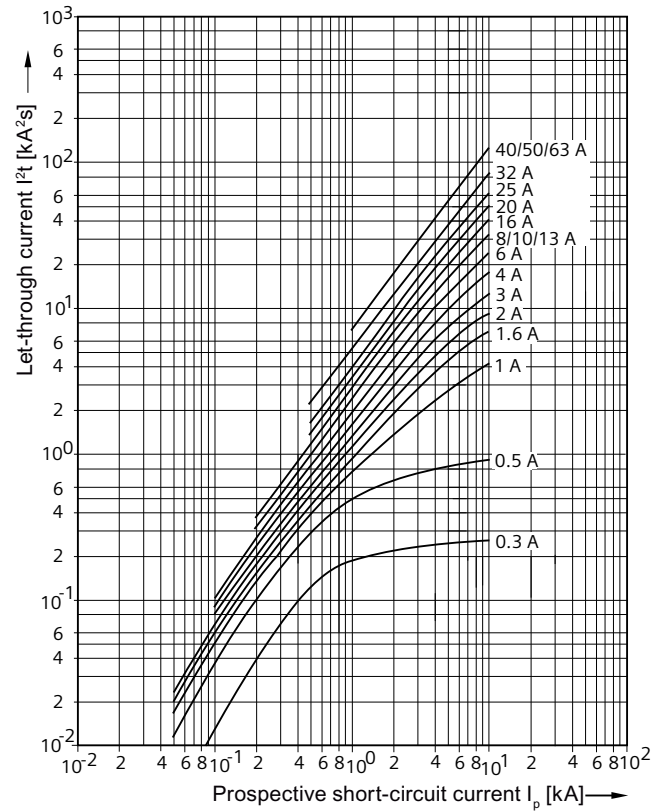
Characteristic D
