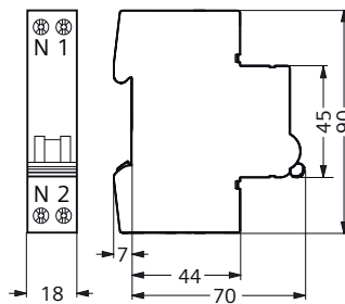
1P+N (N pole, left)
