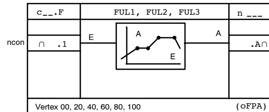
Function transmitter (linear) FUL
