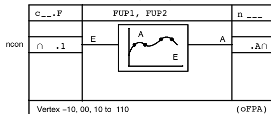
Function transmitter (parabola) FUP
