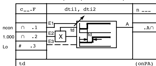
Dead time element dti
