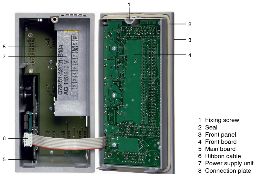
Figure 5-2 Controller with front module open
