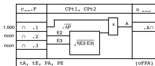
Correction computer pressure, temperature CPT
