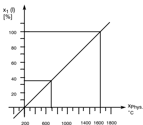
Figure 1-32 Linearized controlled variable x_1(l)
