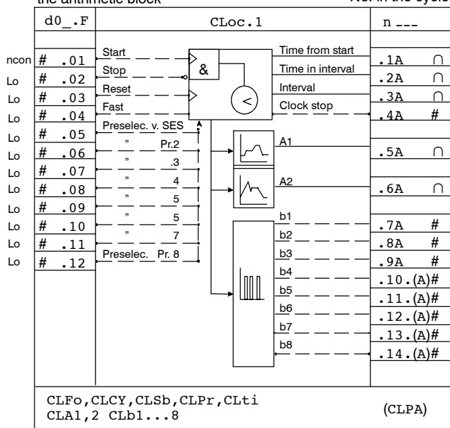
Clock
