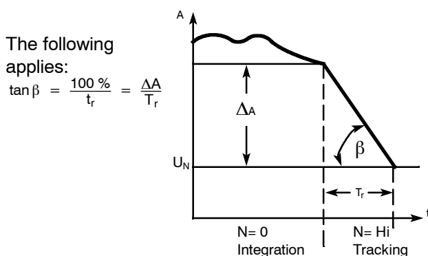
Figure 1-24 Tracking time tr
