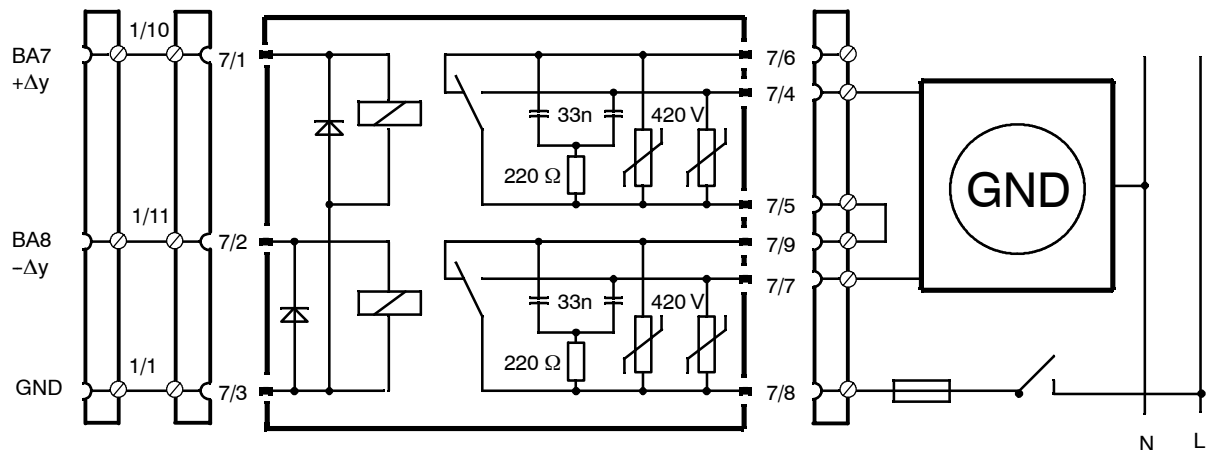
Figure 2-26 Wiring of interface relay 230 V 6DR2804-8B
