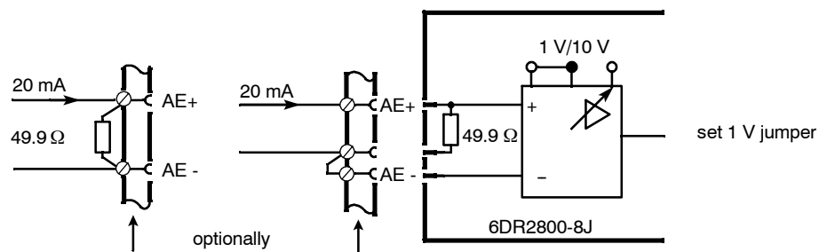
Figure 2-28 Signal input AE4, AE5 via option module 6DR2800-8J, internal or external 49.9\ \Omega resistance
