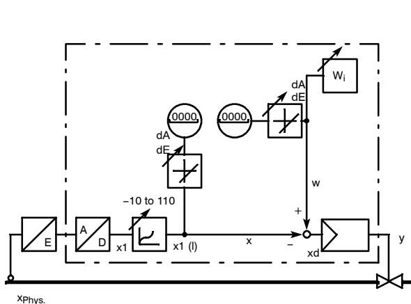
Figure 1-29 Using of function transmitter to linearize non-linear process variables for the display and control
