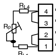
2-wire connection
