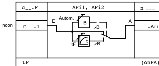
Adaptive filter AFi
