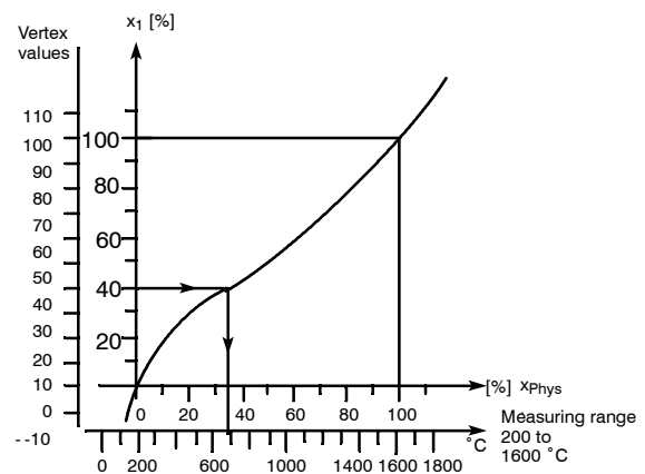
Figure 1-30 Sensor function e.g. from table
