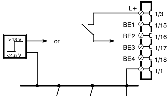
Figure 2-8 BE1 to BE4 wiring diagram
