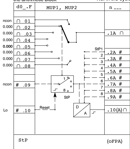
Measuring point switch (multiplexer)
