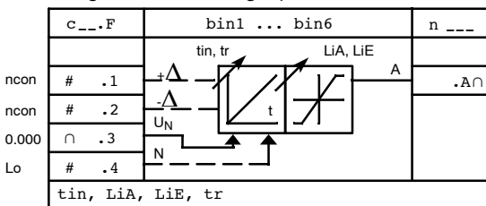
Integrator with binary input bin
