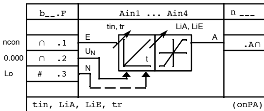
Integrator with analog input Ain
