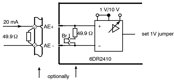
Figure 2-27 Signal input AE1 to AE3 of the standard controller, internal or external 49.9\ \Omega resistance or signal input AE6 to AE8 via module 3AE, 6DR2800-8A
