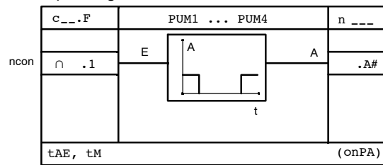
Pulse width modulator
