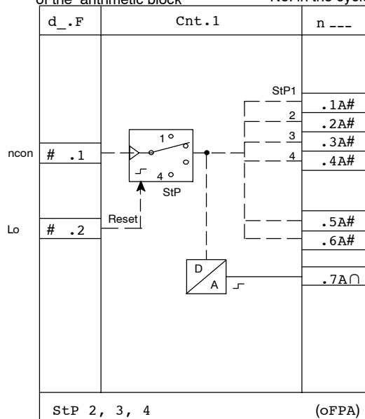
Demultiplexer
