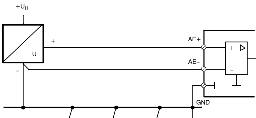
Figure 2-37 Double-pin wiring of a voltage source with positive polarity to ground
