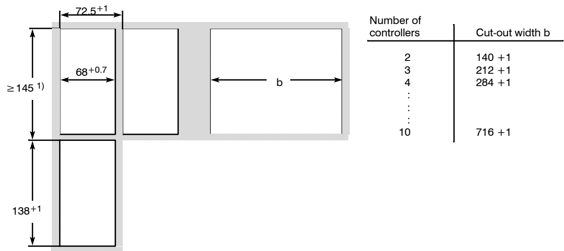
Figure 1-43 Panel cut-outs, dimensions in mm
