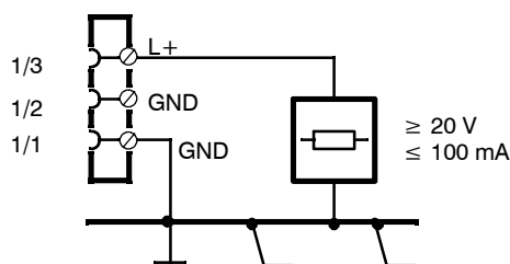
Figure 2-11 L+ connection
