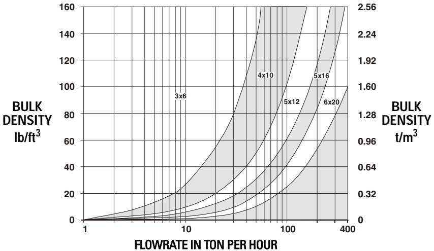
V SERIES FLOWGUIDE CAPACITY CHART
