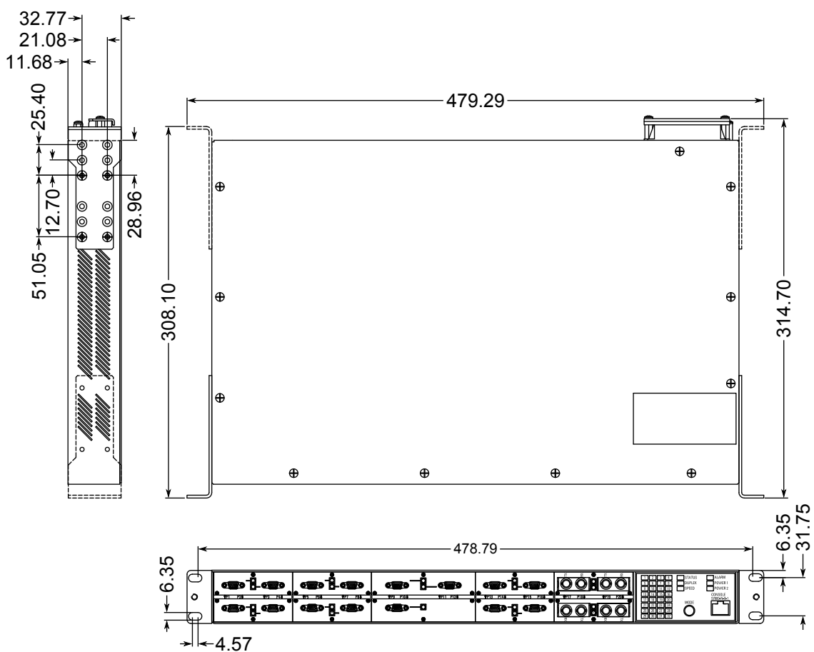
Figure 30: Rack Mount Dimensions
