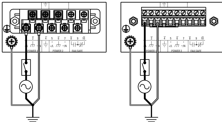
Figure 6: Single AC Power Supply
