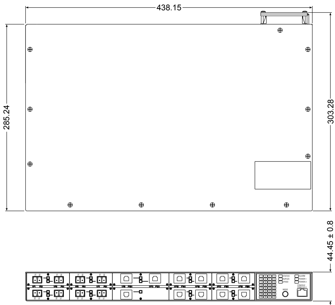
Figure 29: Overall Dimensions
