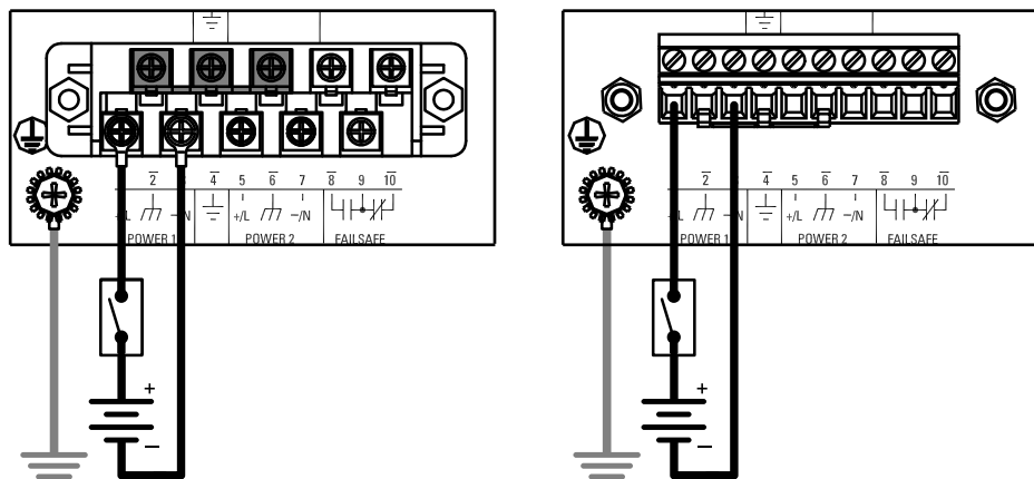
Figure 7: Single DC Power Supply
