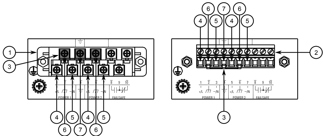
Figure 4: Terminal Block Wiring
