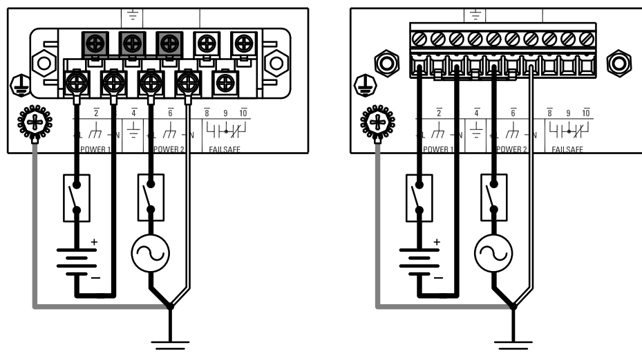
Figure 10: Dual AC/DC Power Supply
