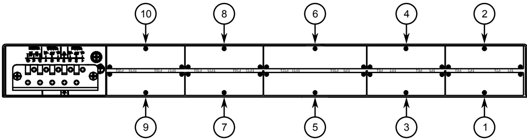
Figure 14: Port Assignment
