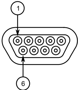
Figure 20: Micro-D 10/100Base-TX Port Pin Configuration
