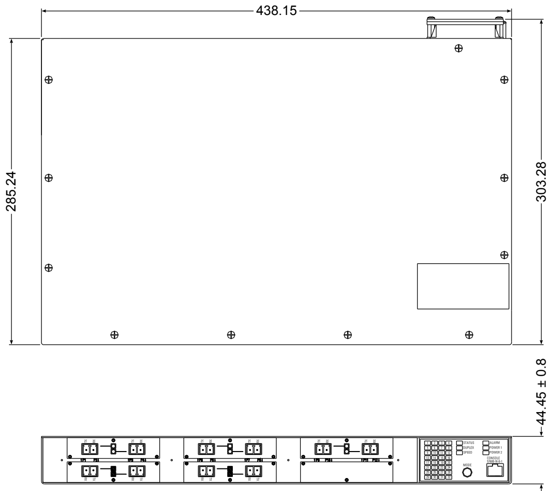
Figure 28: Overall Dimensions
