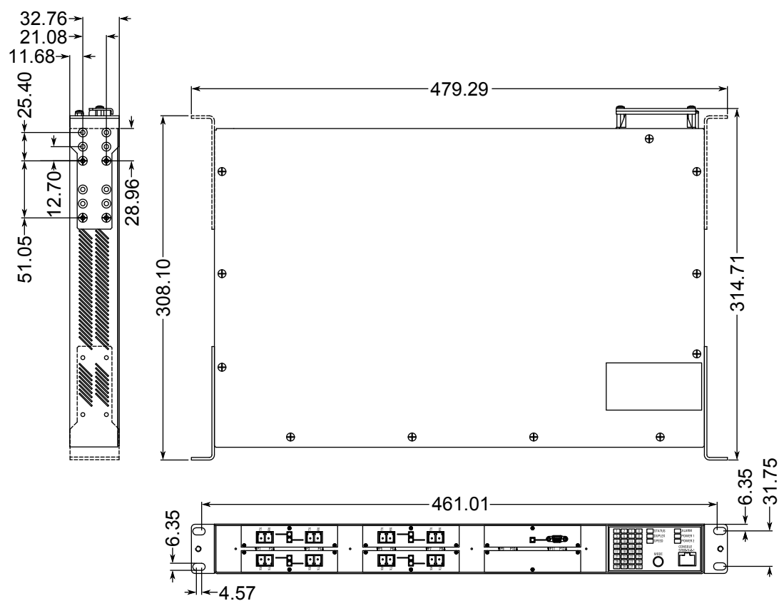
Figure 29: Rack Mount Dimensions
