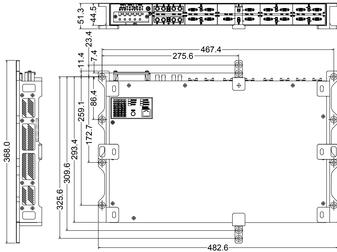
Figure 30: Panel Mount Dimensions
