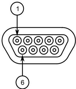
Figure 19: Micro-D 10/100Base-TX Port Pin Configuration
