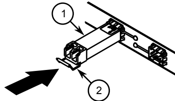
Figure 25: Installing an SFP Optical Port (Typical)
