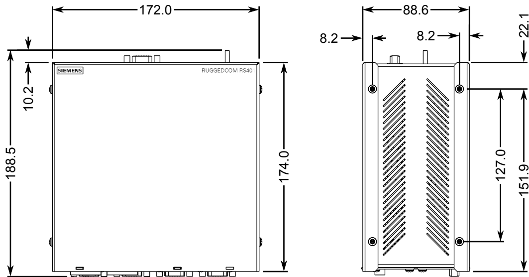
Figure 21: Overall Dimensions
