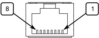
Figure 14: RJ-45 Port Pin Configuration
