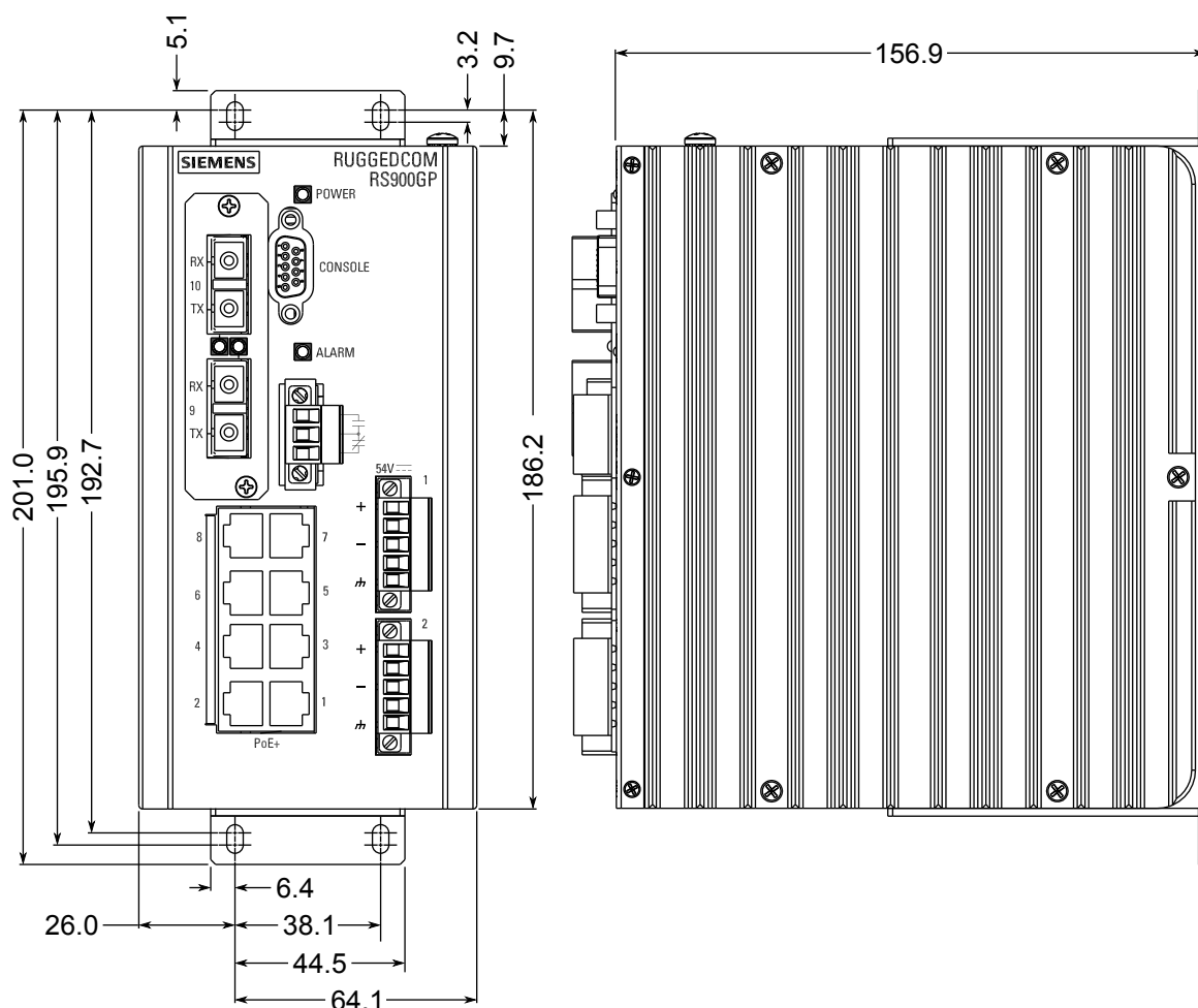
Figure 23: Panel Mount Dimensions (Rear Mount Shown)
