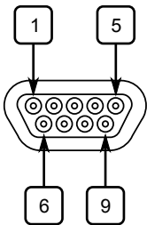
Figure 15: Micro-D Port Pin Configuration
