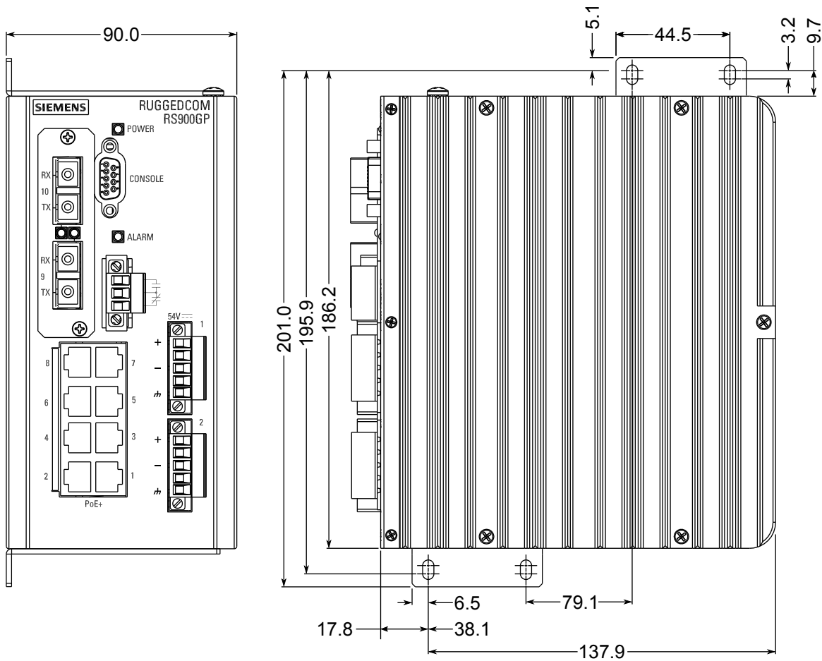
Figure 24: Panel Mount Dimensions (Side Mount Shown)
