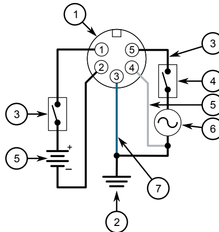
Figure 11: AC and DC Power Supply Wiring Example
