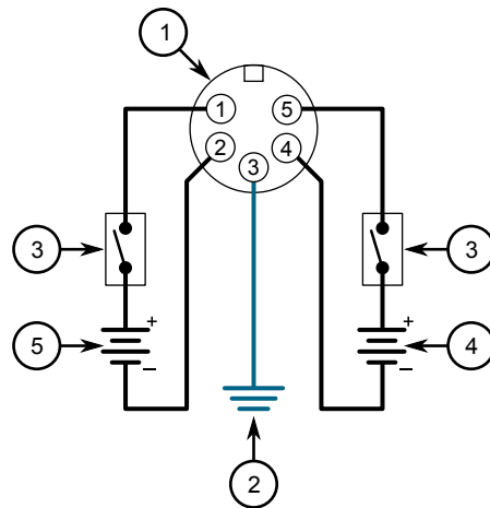
Figure 12: DC and DC Power Supply Wiring Example
