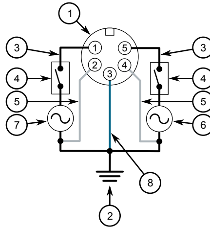
Figure 10: AC and AC Power Supply Wiring Example
