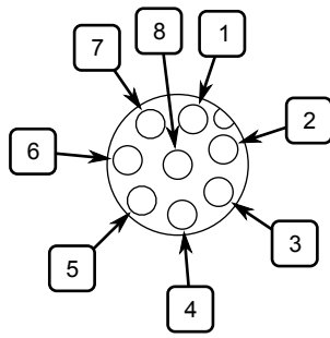
Figure 15: M12 Console Port Pin Configuration
