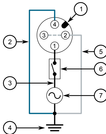
Figure 6: AC Power Supply Wiring Example (Mini Power Connector)
