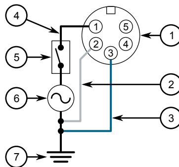
Figure 7: AC Power Supply Wiring Example (M23 Power Connector)
