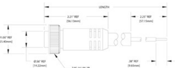
Figure 25: Mini Power Mating Cordset
