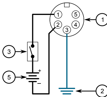
Figure 9: DC Power Supply Wiring Example (M23 Connector)
