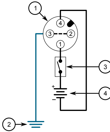
Figure 8: DC Power Supply Wiring Example (Mini-Change Connector)
