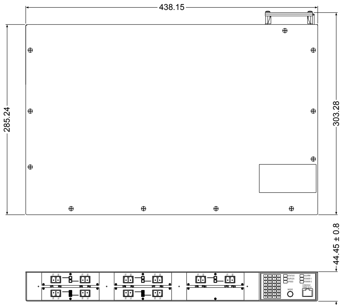
Figure 32: Overall Dimensions
