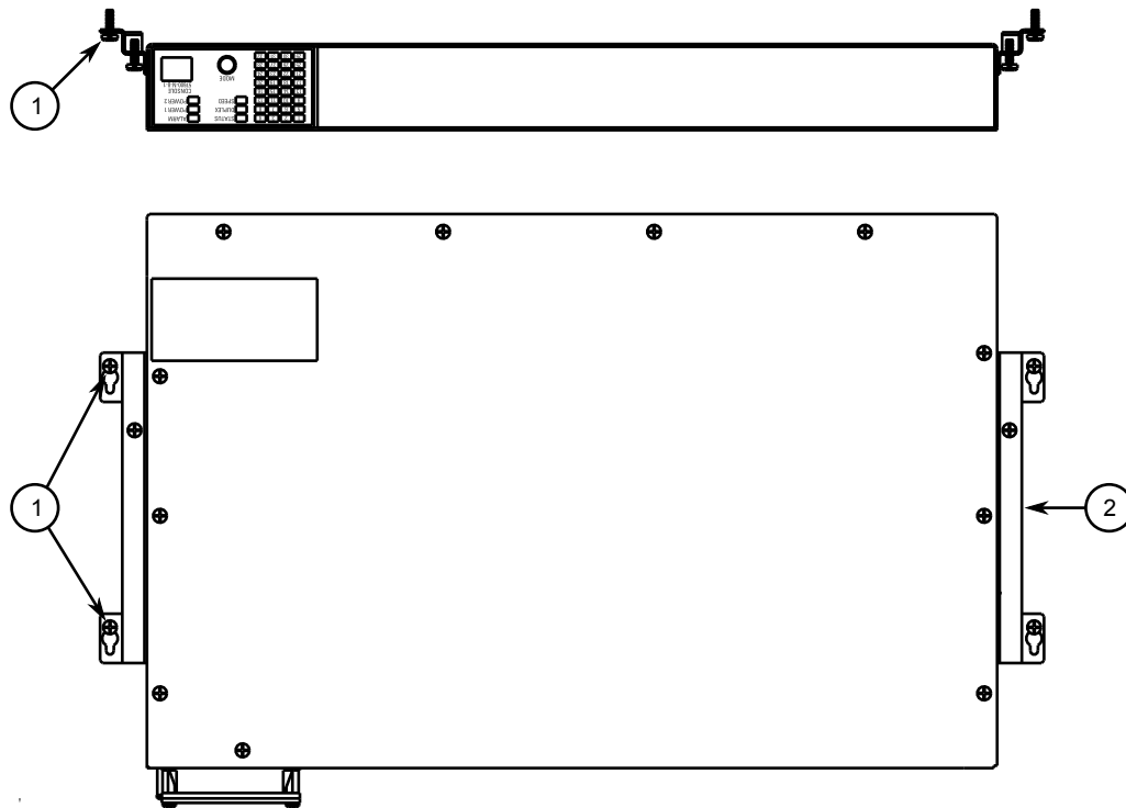
Figure 4: Panel Mounting
