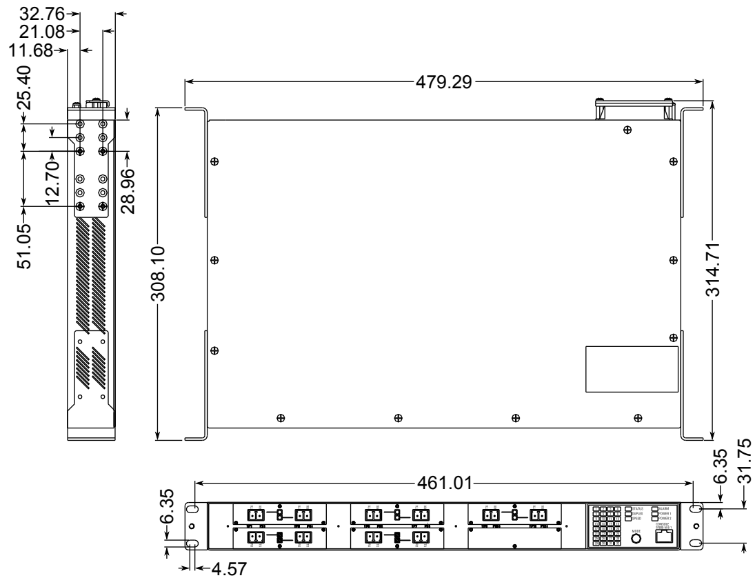
Figure 33: Rack Mount Dimensions
