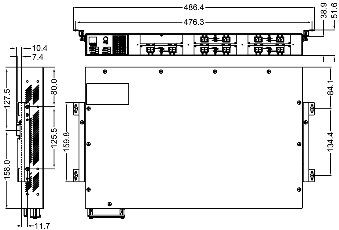
Figure 34: Panel and DIN Rail Mount Dimensions
