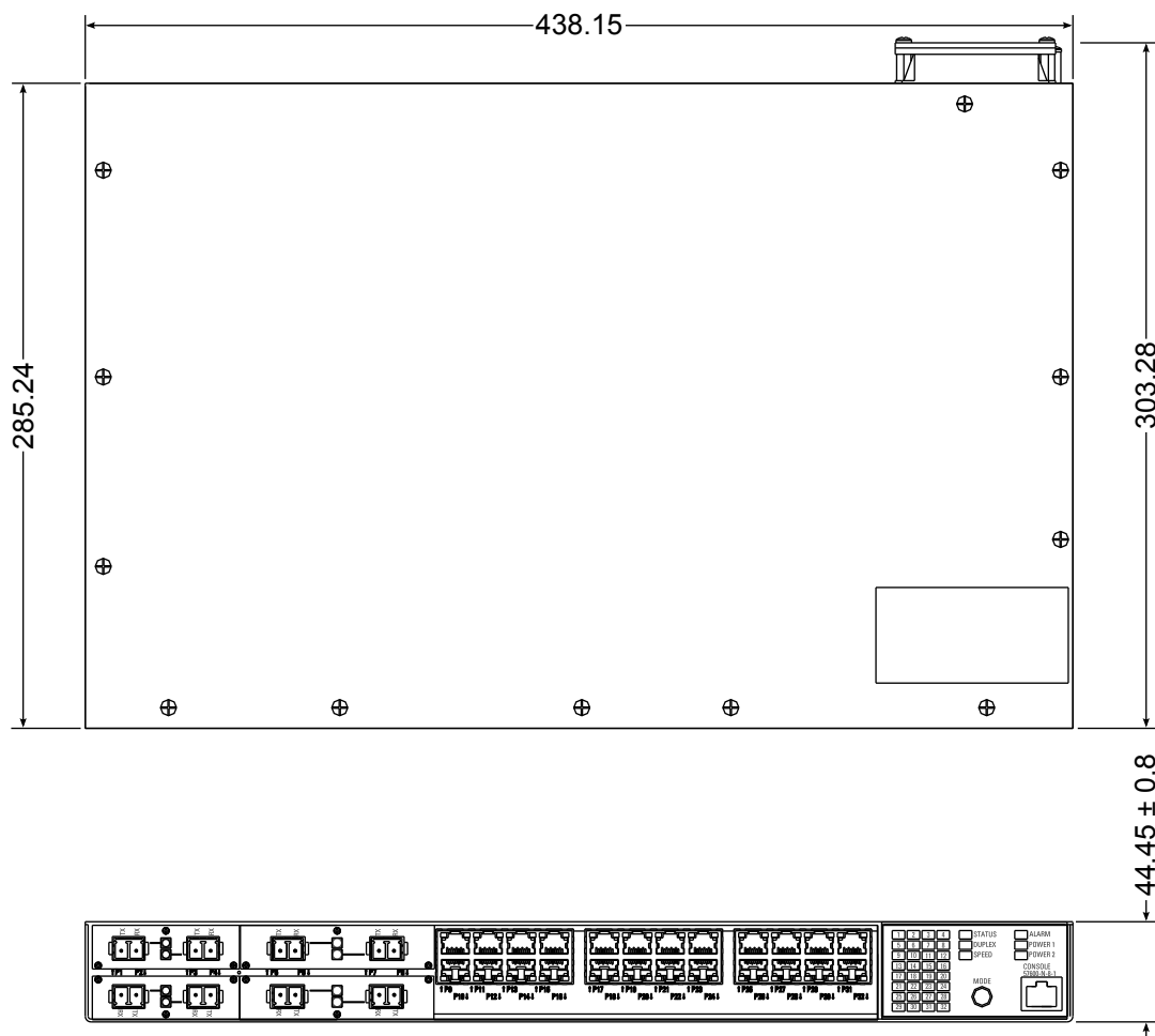
Figure 33: Overall Dimensions
