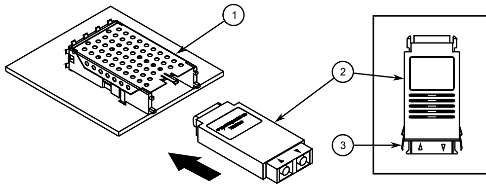
Figure 30: Installing a GBIC Optical Port
