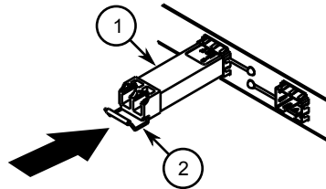
Figure 27: Installing an SFP Optical Port (Typical)
