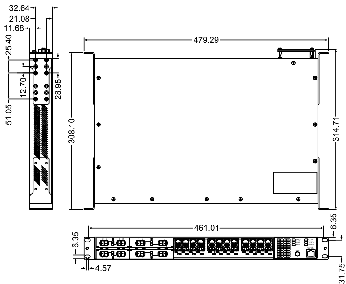
Figure 34: Rack Mount Dimensions
