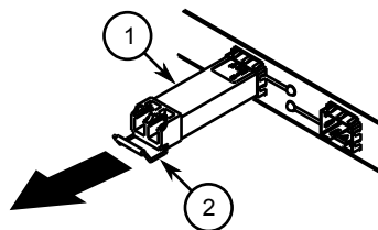
Figure 28: Removing an SFP Optical Port (Typical)
