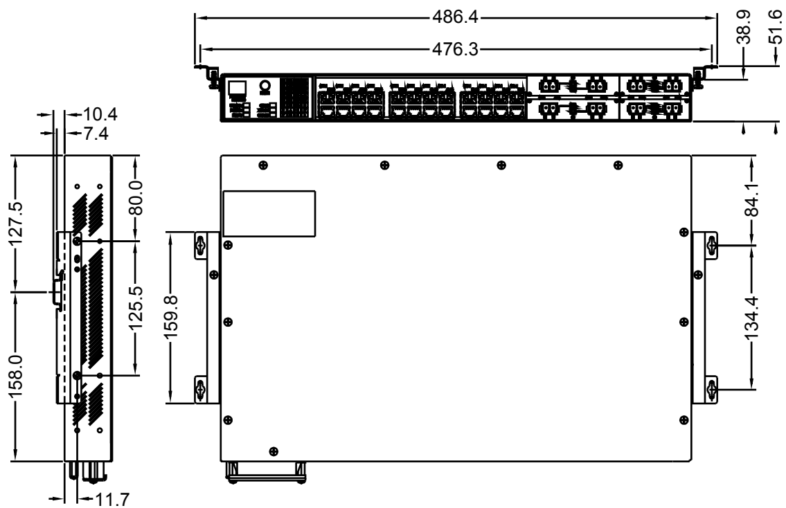
Figure 35: Panel and DIN Rail Mount Dimensions
