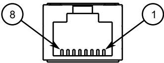
Figure 26: Serial RJ45 Port Pin Configuration
