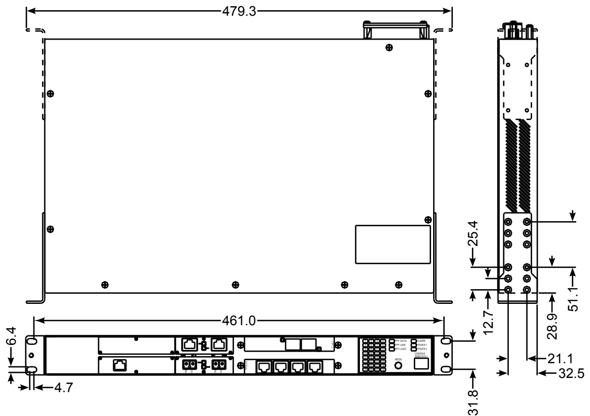
Figure 35: Rack Mount Dimensions
