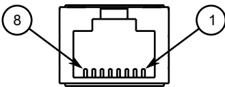
Figure 21: RJ45 T1/E1 Port Pin Configuration
