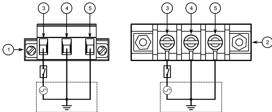
Figure 7: AC Terminal Block Wiring
