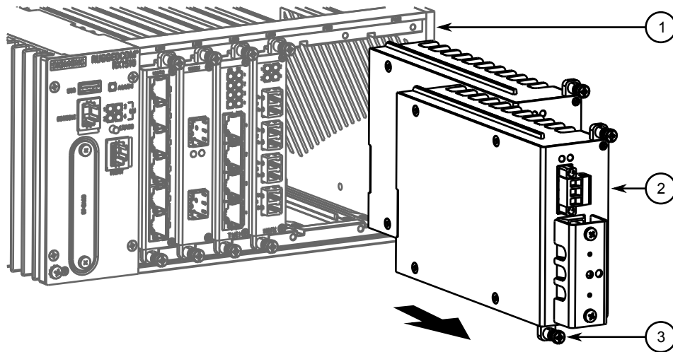
Figure 6: Removing a Power Supply
