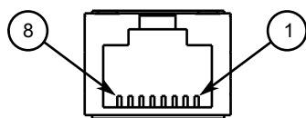
Figure 11: RJ-45 Console Port Pin Configuration
