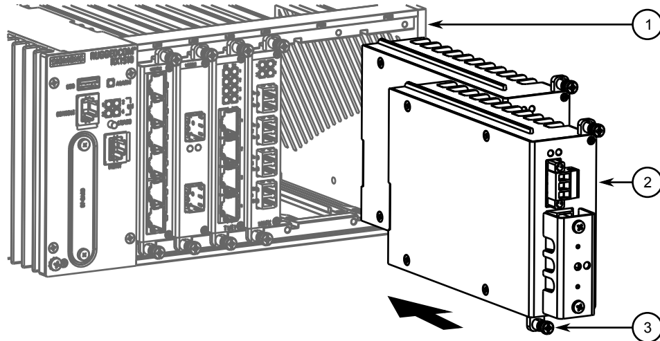
Figure 5: Installing a Power Supply
