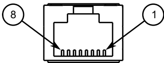
Figure 41: RJ45C T1/E1 Pin Configuration
