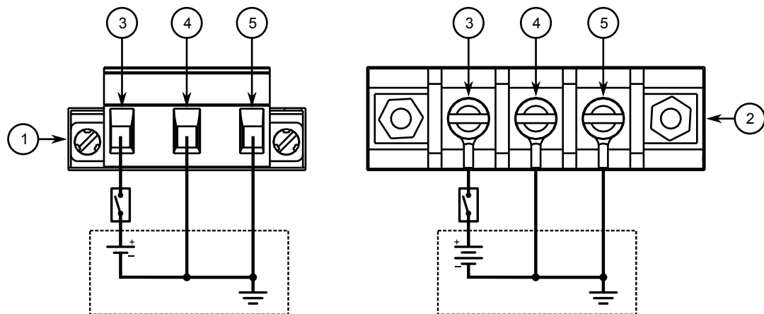
Figure 8: DC Terminal Block Wiring
