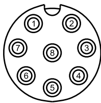
Figure 25: 8-Pin M12 A-Coded Ethernet Port Pin Configuration
