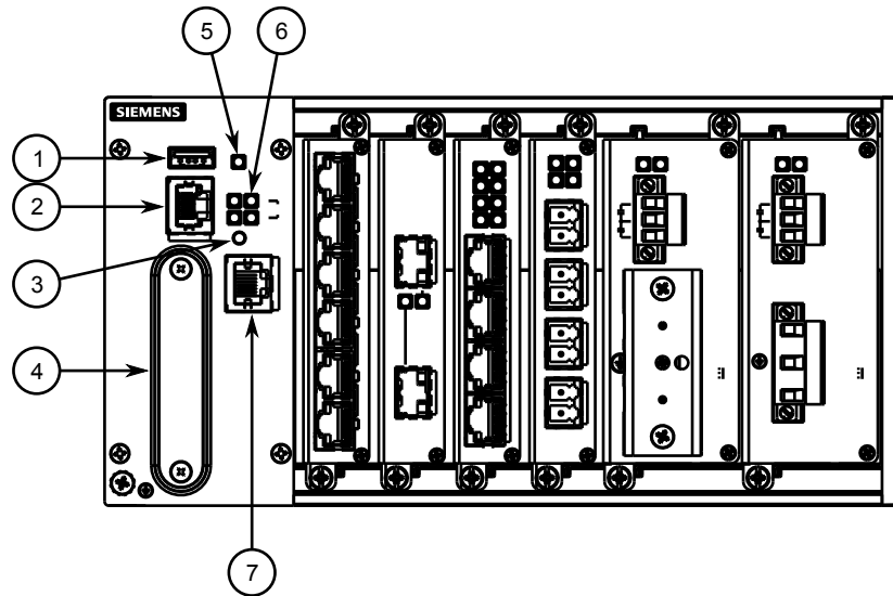
Figure 1: RUGGEDCOM RX1510
