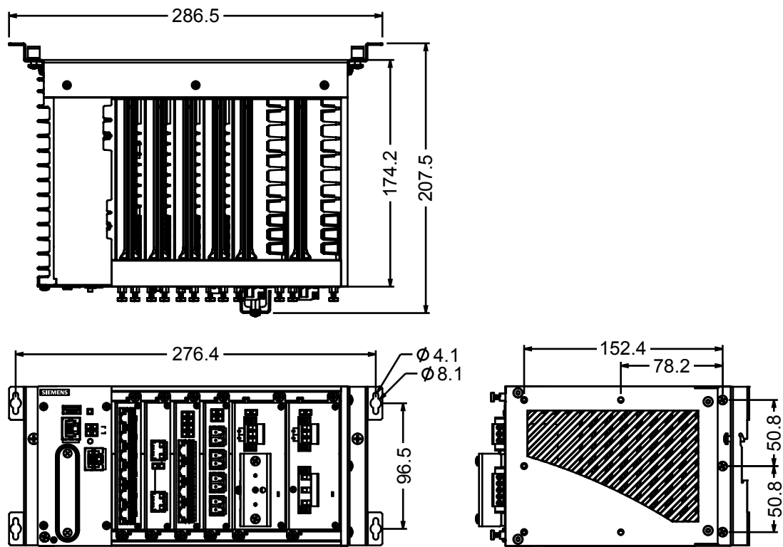
Figure 54: Panel and Din Rail Mount Dimensions
