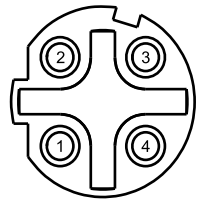
Figure 27: 4-Pin M12 D-Coded Ethernet Port Pin Configuration
