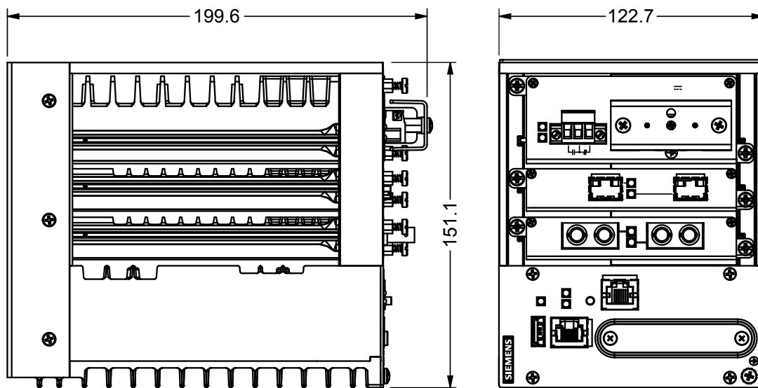
Figure 53: Overall Dimensions
