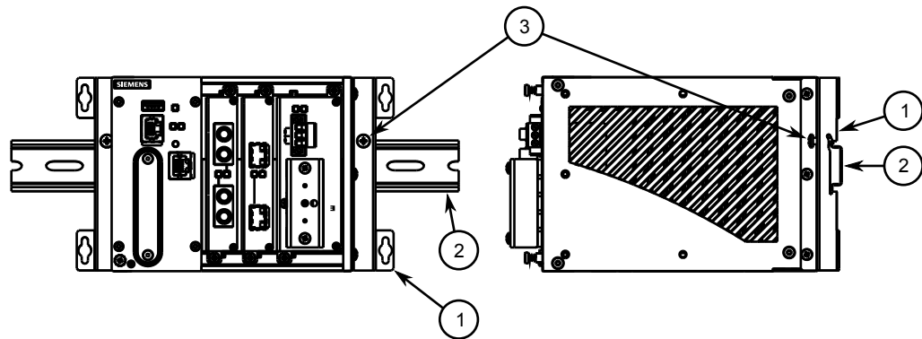
Figure 2: DIN Rail Mounting
