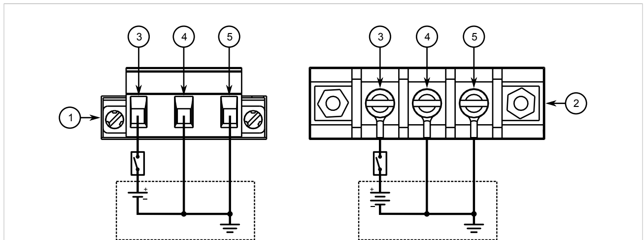
Figure 8: DC Terminal Block Wiring
