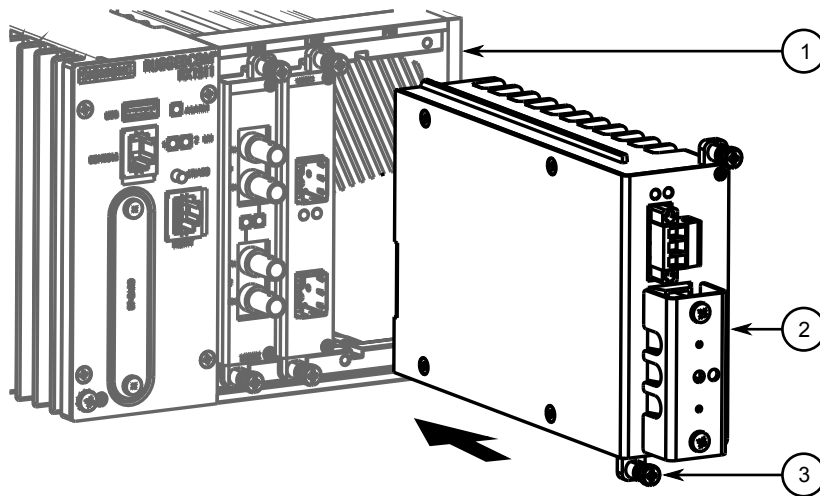
Figure 5: Installing a Power Supply
