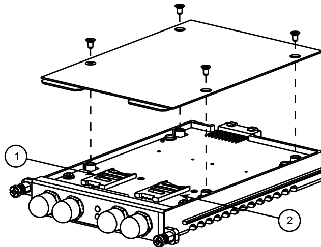
Figure 46: W12, W22, W32 Cellular Modem
