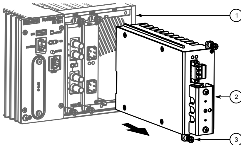
Figure 6: Removing a Power Supply
