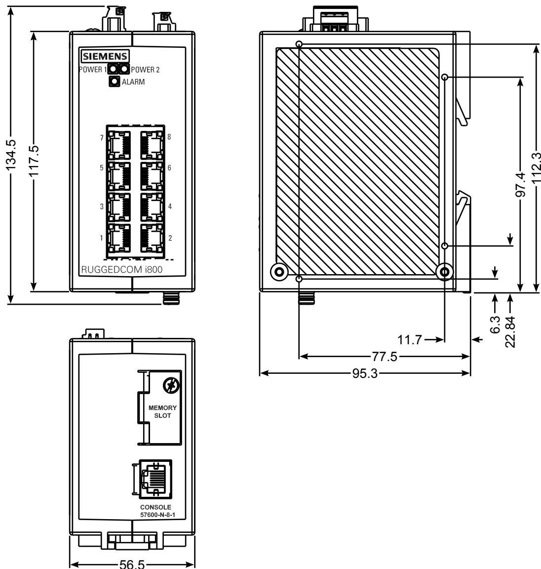
Figure 10: Overall Dimensions
