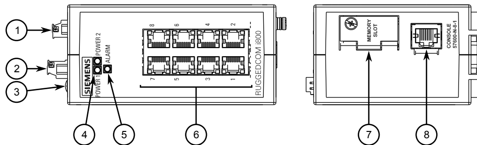
Figure 1: RUGGEDCOM i800
