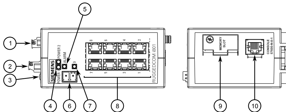
Figure 1: RUGGEDCOM i801
