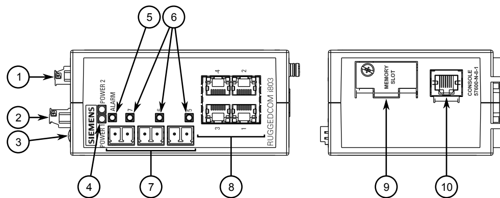
Figure 1: RUGGEDCOM i803
