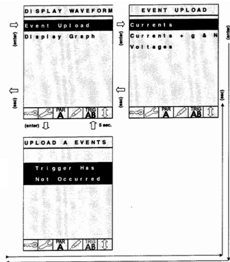
Event Upload – Загрузка события; Currents - Токи; Trigger Has Not Occurred – Запуск не произошел
