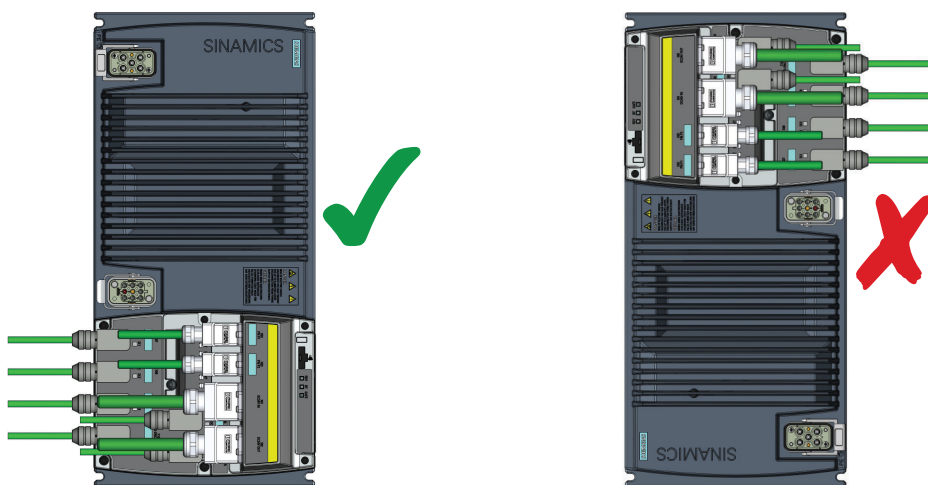
Vertical mounting
